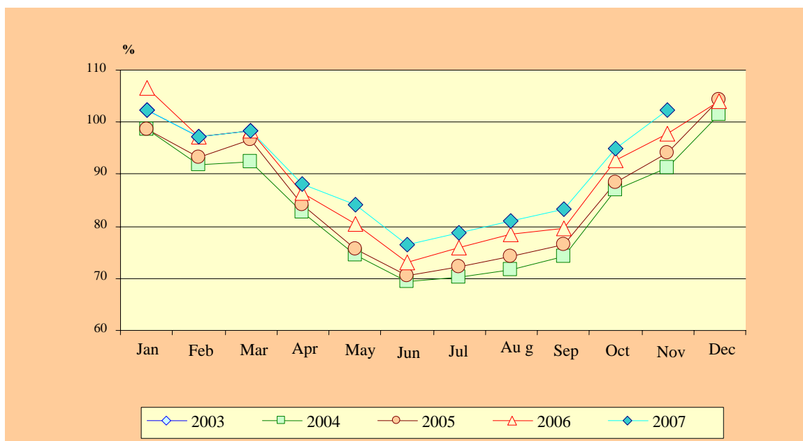
Electric power production growth rates (December of 2001 – 100%)
